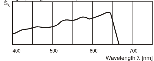
Relative spectral sensitivity (wedge spectrogram at 2850 K)
